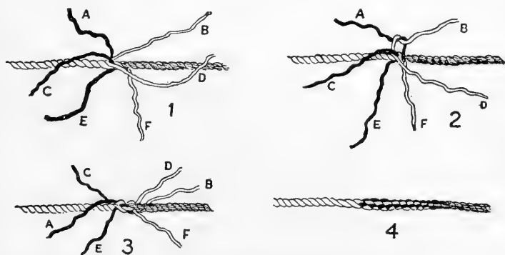
FIG. 231.—Short splice, showing four stages in the operation. 1. The six strands of the two ropes arranged in pairs, A-B, C-D, E-F. 2. A-B tied with first overhand knot. 3. Each of the three pairs tied with first step of surgeon's knot. 4. Completed splice.
